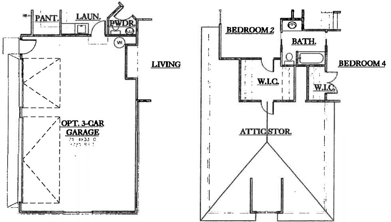
OPT. 3-CAR GARAGE PLAN (1ST. & 2ND.)
